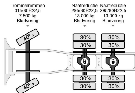
Renault R385 Major 6x4 SPRING SUSPENSION/LAMME (ZF...
