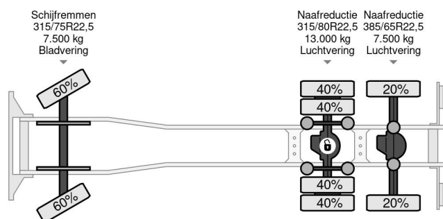
MAN 26.414 FNL-T (6-CILINDERHEADS) 6x4 CHASSIS (EU...
