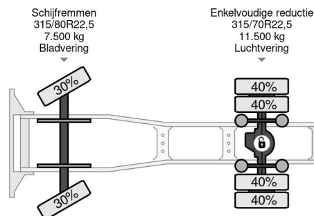
Renault Magnum AE 480 DXI (MANUAL GEARBOX / ZF... 4x2 Referentienummer: SN 58740690 Z
