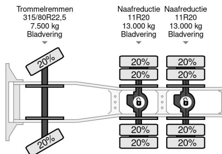
MAN 26 240DFS FULL STEEL SUSPENSION / DAYCA... 6x4
