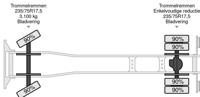
Mercedes-Benz LK 814 RECOVERY TRUCK / CAR-MA... 4x2
