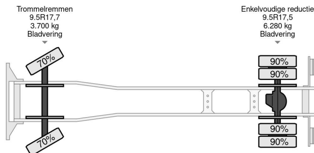
Mercedes-Benz LK 914 (6-CILINDER) WITH TENT BOX... 4x2
