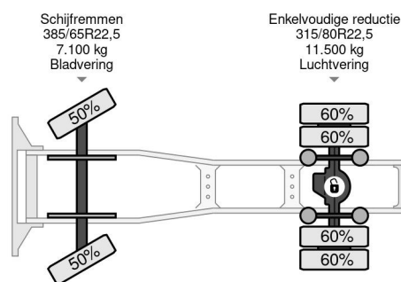
Volvo FH 440 GLOBETROTTER-XL (I-SHIFT / ENGINE... 4x2
